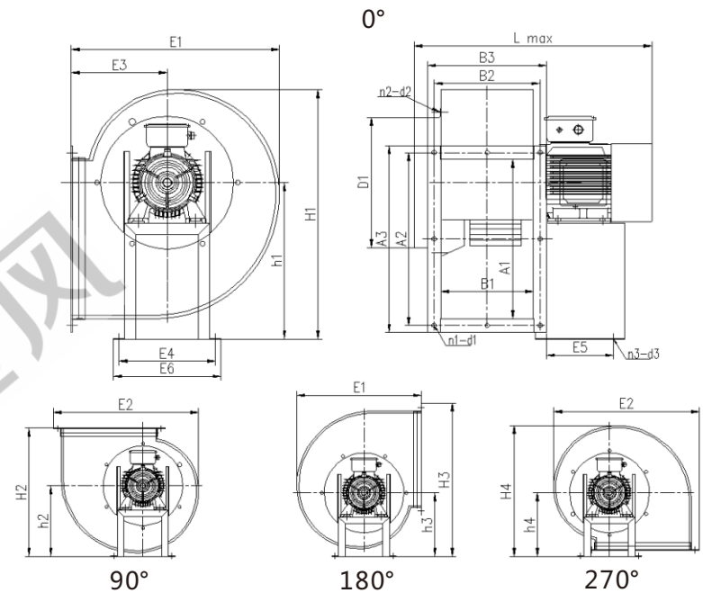
进出风口尺寸 Inlet and outlet dimensions
